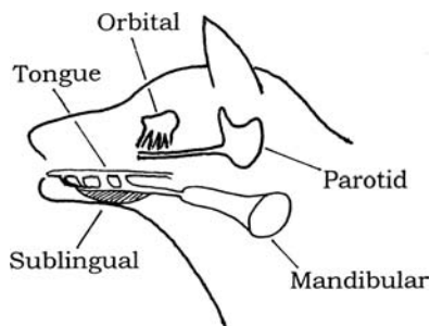
FIGURE 4.6. Salivary glands of the wolf.
