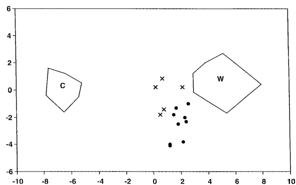
FIGURE 9.6. Statistical distribution of four groups of female Canis , based on the first (horizontal axis) and second (vertical axis) canonical variables, as produced by a canonical discriminant analysis of ten skull measurements. Solid lines represent the limits of eighteen western C. latrans (letter C shows mean) and twenty Minnesota C. lupus (letter W shows mean); solid circles, nine C. rufus taken 1919–1924 in southeastern Missouri; X's, five suspected hybrids of C. latrans and C. lupus from southeastern Canada. (Cf. Nowak 1995b and Jenks and Wayne 1992.)
