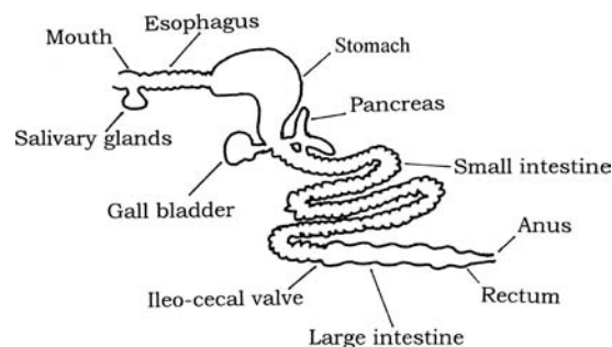
FIGURE 4.7. Digestive anatomy of the wolf.
